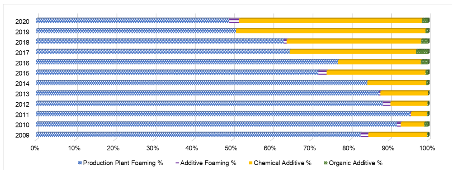
Figure 18: WMA Technologies Used as Percent of WMA Production, 2009–2020
